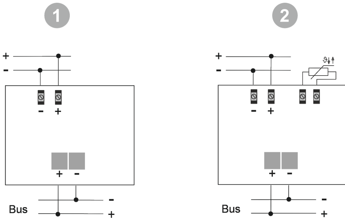
Fig. 9: Electrical connection
