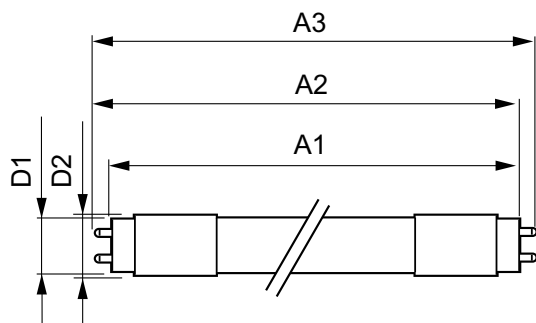
TLED T8 220-240V 21.8-58W 3700lm 6500K
