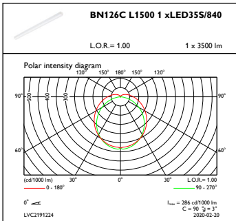
OFPC1_BN126CL15001xLED35S840
